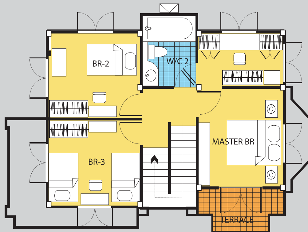
SECOND FLOOR
